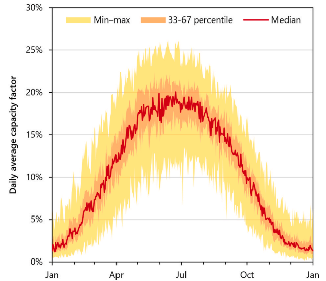
Fig. 3. The temporal variability in solar PV capacity factors in the UK. Daily average capacity factor is summarized over 30 years, highlighting the range over the seasons and variability between years. Capacity factors modelled using the Renewables.ninja software [29]. Reproduced from Ref. [30].
