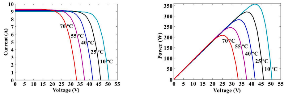
Fig. 9. Solar cell I-V and P-V curves at different temperatures at a constant irradiance intensity of 1000 \text{ W/m}^2 [39]. (left) shows that temperature has a stronger effect on open-circuit voltage than the increase in short-circuit current. (right) shows that power output decreases near-linearly with temperature [39].
