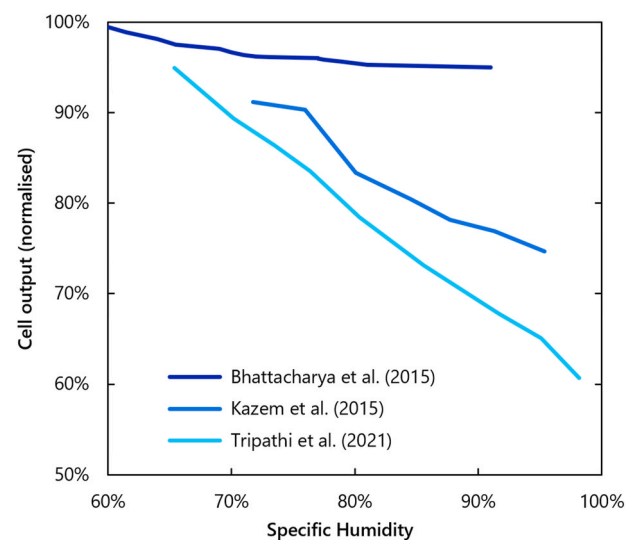
Fig. 17. Variation of PV module efficiency with humidity. Data from Refs. [165–167].
