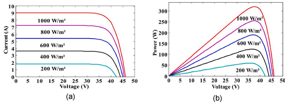
Fig. 5. Solar cell I-V and P-V curves at different irradiance intensities at a constant temperature of 25°C [39]. (a) shows that irradiance has a stronger effect on short-circuit current than on open-circuit voltage. (b) shows that power output increases near-linearly with irradiance.
