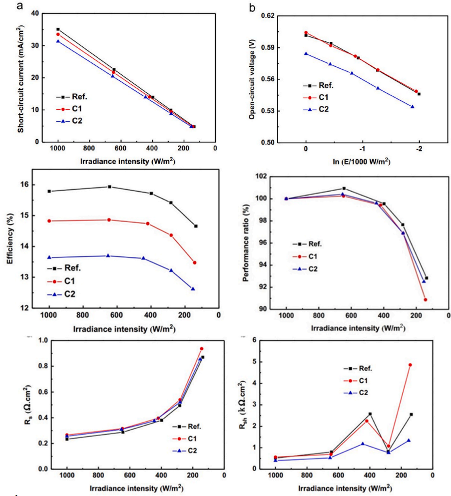
Fig. 6. Relationships between irradiance and various operating parameters of solar cells [40]. (a) shows the linear relationship for short-circuit current density, (b) shows the logarithmic relationship for open-circuit voltage, (c) and (d) show the relationship with efficiency and performance ratio. (e) shows series resistance ( R_s ) and (f) shows shunt resistance ( R_{sh} ), which decrease with irradiance [40]. Lines refer to a standard reference B-doped silicon crystal (Ref.), and compensated silicon crystals created with electronic grade silicon doped with boron (C1) and phosphorus (C2).
