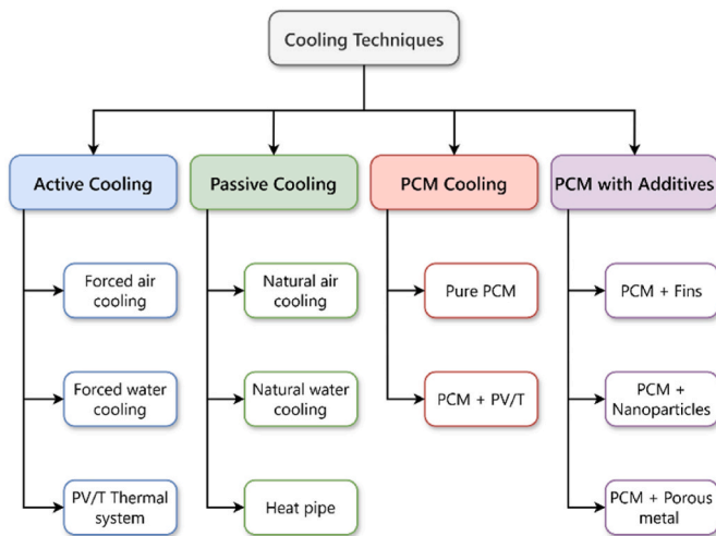
Fig. 12. Classification of different PV module cooling methods, based on [87]. PCM: phase change material; PV/T: photovoltaic/thermal.
