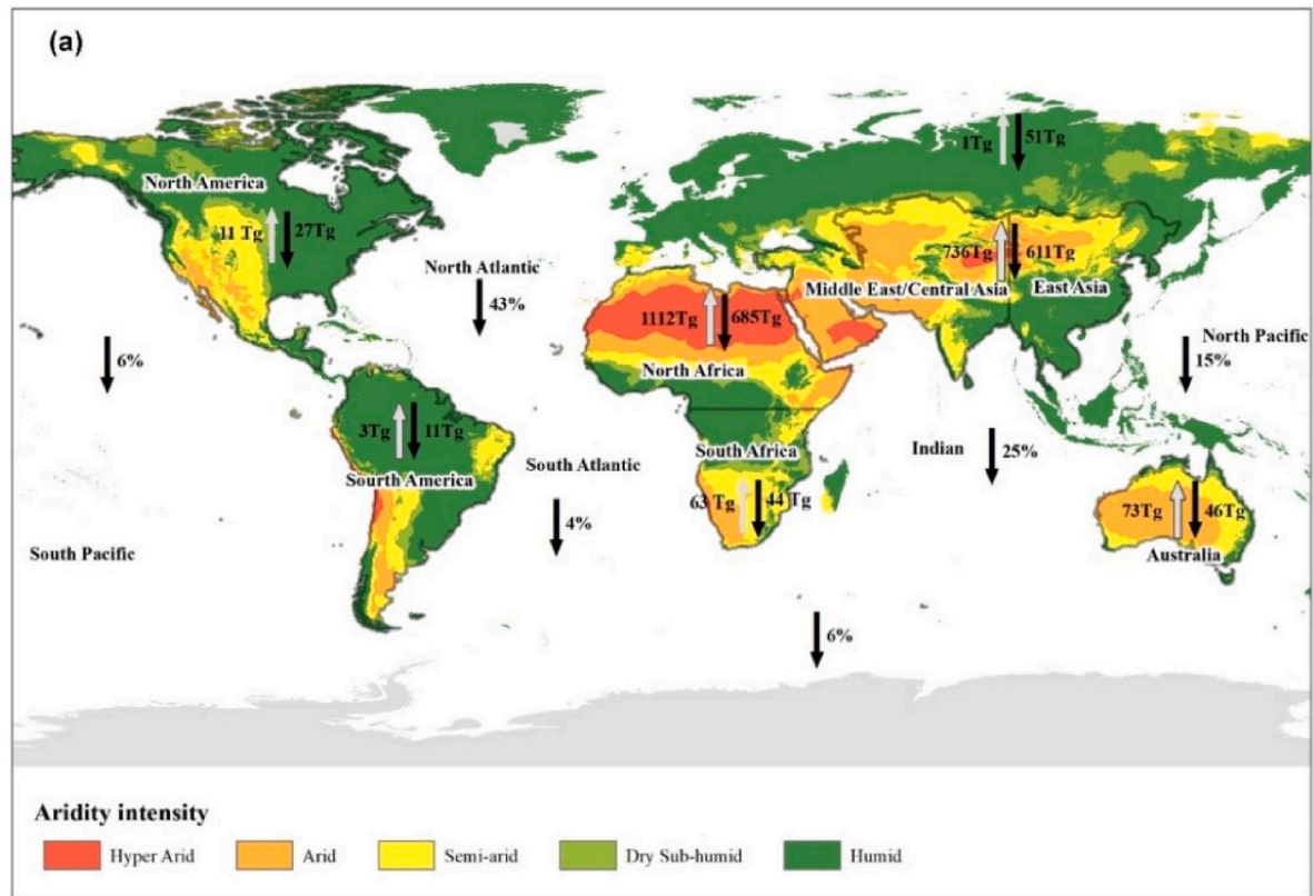
Fig. 14. Global map of dust emissions and deposition. Grey and black arrows indicate dust emission and deposition respectively, as shares of the total global dust cycle [113].
