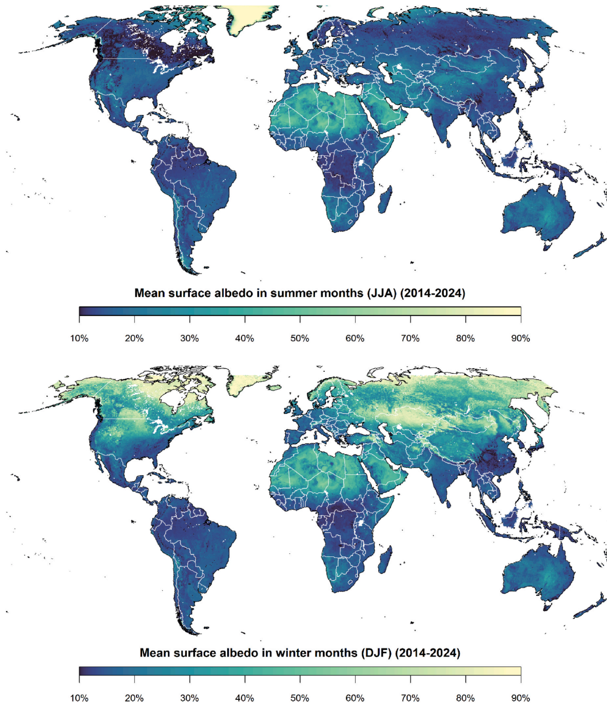
Fig. 18. Global maps of average albedo in summer (top panel) and winter months (bottom panel). Measurements are averaged over the months of June, July and August 2014–2024 for summer, and December, January and February 2014–2024 for winter. Darker colours indicate surfaces with lower light reflection, and bright white areas indicate no data, due to water coverage. Data from Ref. [185].
