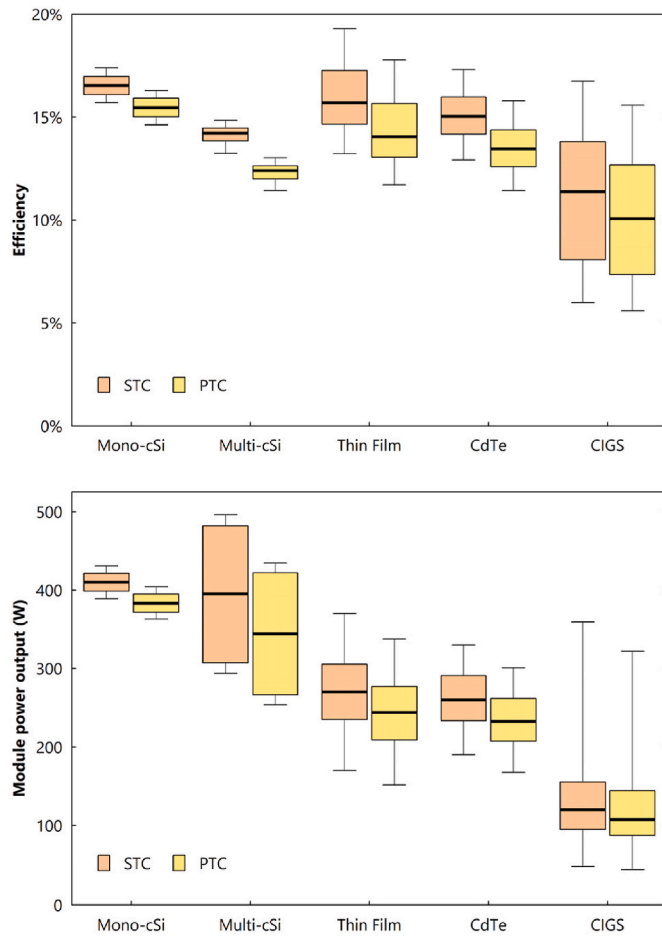
Fig. 2. Summary of the conversion efficiency and power output of 21,000 commercially-available solar PV modules, aggregated by cell technology. Parameters are measured using the STC and PTC standards. Data from the CEC database [17]. The thick line denotes the median coefficient, the shaded area denotes the interquartile range, and whiskers extend to the 5th and 95th percentiles. Mono-cSi: monocrystalline silicon ( n = 9614 ); Multi-cSi: Multicrystalline silicon ( n = 11,174 ); Thin film ( n = 561 ); CdTe: Cadmium Telluride ( n = 20 ); CIGS: Copper Indium Gallium Selenide ( n = 8 ).
