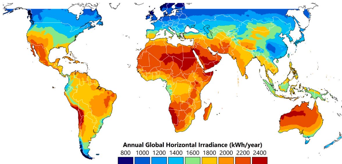
Fig. 4. The geographical variation in global horizontal irradiance (GHI) from 1994/1999/2007 (depending on the location) to 2018 [31].
