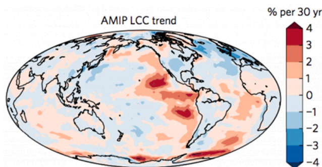
Fig. 22. The global change in low-level cloud cover from 1980 to 2005. Shading depicts increase (red) and decrease (blue) in cloud cover [260].
