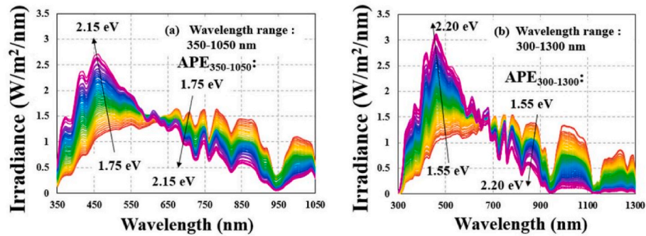
Fig. 7. Spectral irradiance with different APE values. Spectral irradiances in two wavelength bands with varying APE values: 350–1050 nm and 300–1300 nm. Total irradiances in these wavelength ranges were 792 and 923 \text{W/m}^2 . APE: Average Photon Energy [47].
