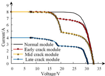
Fig. 19. Damage to PV modules caused by hail in Nebraska, US (left), and the I-V characteristics of cracked PV modules (right). Lines represent the progression of a module’s performance over time: ‘normal’ refers to a module with no cracks, ‘early’ is 3 months, ‘mid’ is 6 months, and ‘late’ is 12 months after cracking occurred. Photo courtesy of GenPro Energy Solutions [227], chart reproduced from Ref. [226].
