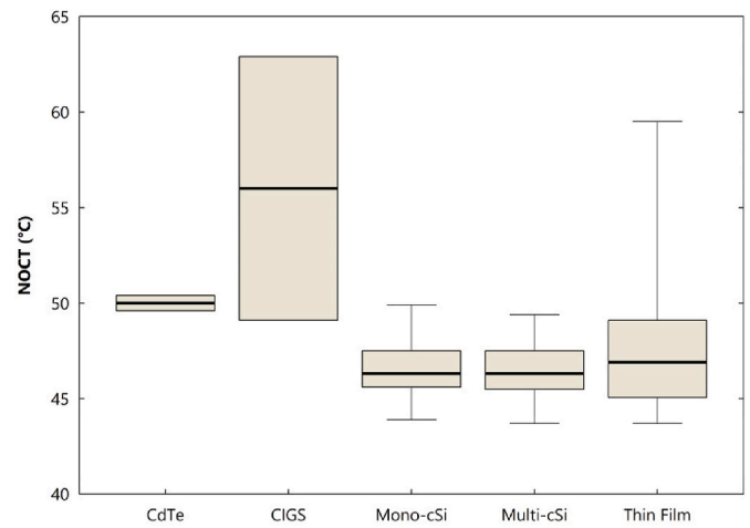
Fig. 11. The Nominal Operating Cell Temperature (NOCT) for 21,000 commercially-available solar PV modules, aggregated by cell technology. Data from the CEC database [17]. Figure design and nomenclature is the same as for Fig. 10.
