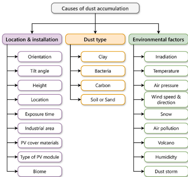
Fig. 15. Classification of the factors affecting dust accumulation on solar PV modules, based on [114].
