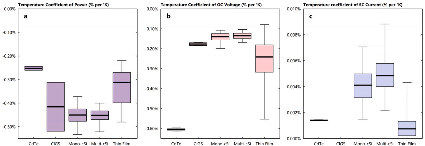
Fig. 10. Summary of the temperature coefficients from 21,000 commercially-available solar PV modules, aggregated by cell technology. Coefficients are given for (a) maximum power production, (b) open-circuit voltage, and (c) short-circuit current. Data from the CEC database [17]. The thick line denotes the median coefficient, the shaded area denotes the interquartile range, and whiskers extend to the 5th and 95th percentiles. CdTe: Cadmium Telluride ( n = 20 ); CIGS: Copper Indium Gallium Selenide ( n = 8 ); Mono-cSi: monocrystalline silicon ( n = 9614 ); Multi-cSi: Multicrystalline silicon ( n = 11,174 ); Thin film ( n = 561 ).
