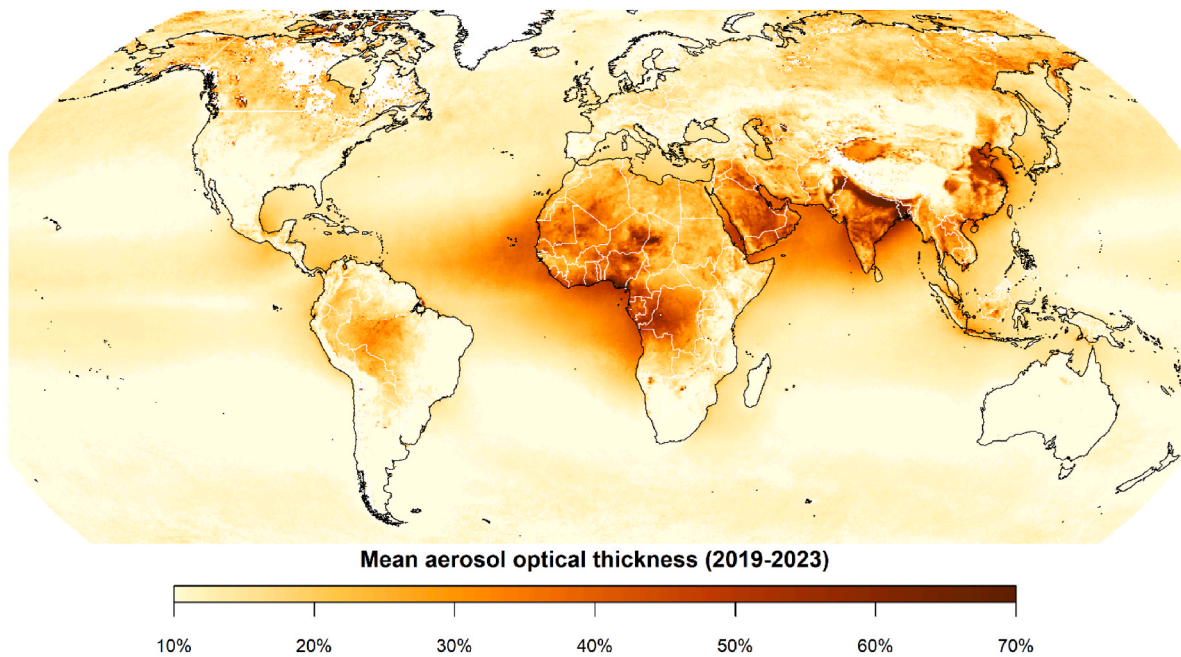
Fig. 13. Global map of aerosol optical thickness averaged over January 2019 to December 2023. Darker areas indicate higher aerosol levels, white patches indicate no data. Data from Ref. [109].
