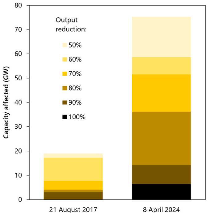
Fig. 20. Utility-scale solar PV capacity in the US affected by solar eclipses in 2017 and 2024. Data from Refs. [234,235].
