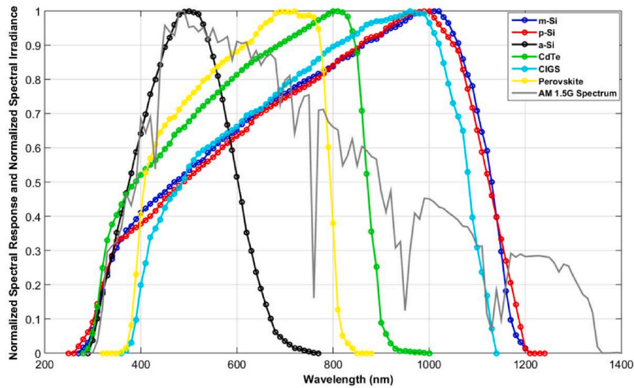
Fig. 8. The different spectral response characteristics of various solar module technologies. m-Si: monocrystalline silicon; p-Si: polycrystalline silicon; a-Si: amorphous silicon; CdTe: cadmium-telluride; CIGS: copper indium gallium selenide sulphide; AM 1.5G: Air Mass 1.5 global spectrum [48].
